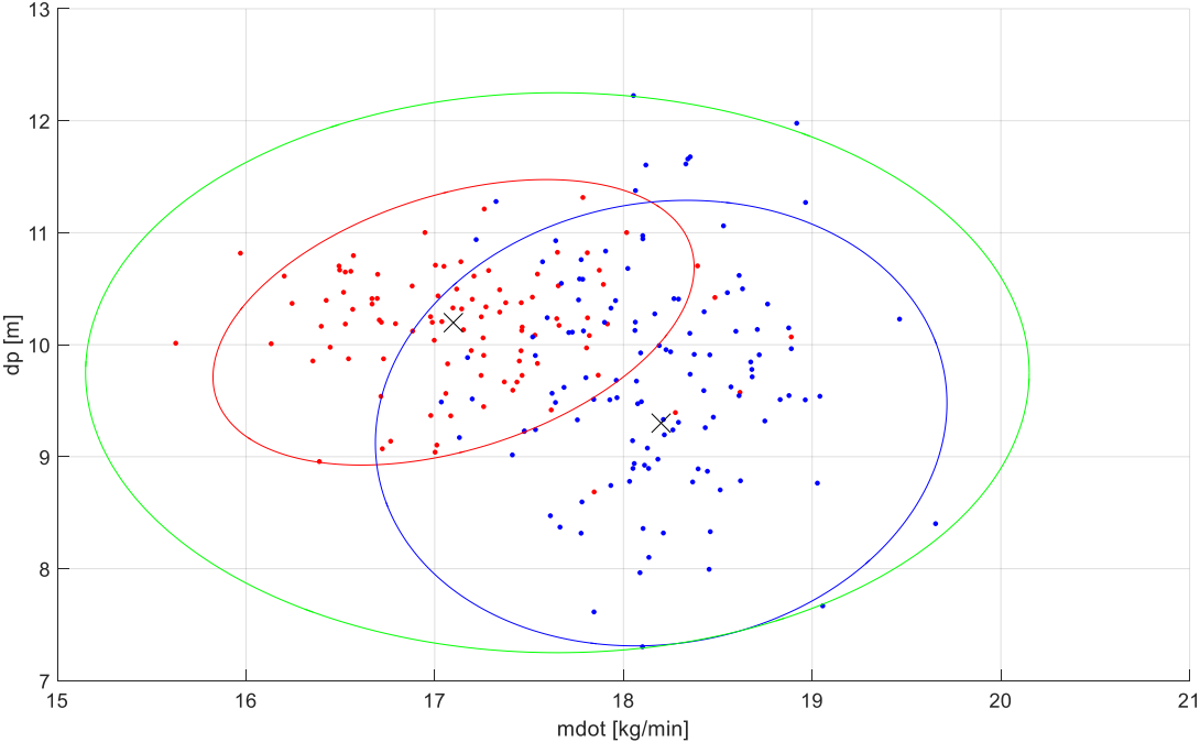
Figure 1: Reference Test - n=1000, valve_pos=0.7, Group1=PS-13/AK (red), Group2=PS-15/AK (blue); green="good-range"
